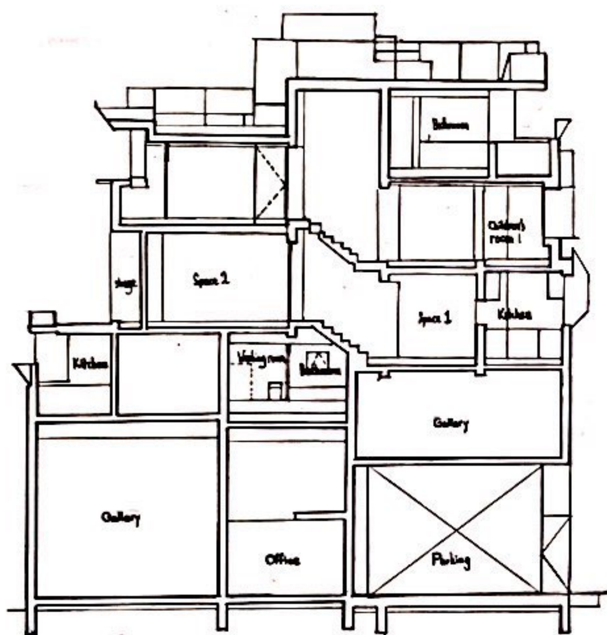
C-C Section
