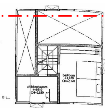
2nd floor plan(upper); scale: 1/150
