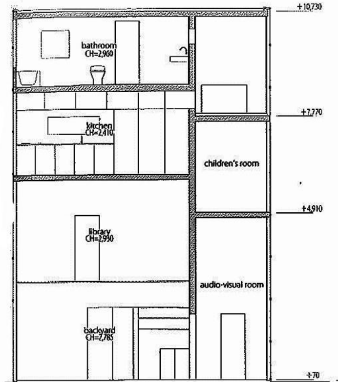
C-C section; scale: 1/150
