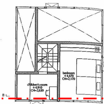
2nd floor plan(upper); scale: 1/150
