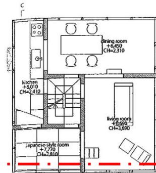
3rd floor plan (lower); scale: 1/150
