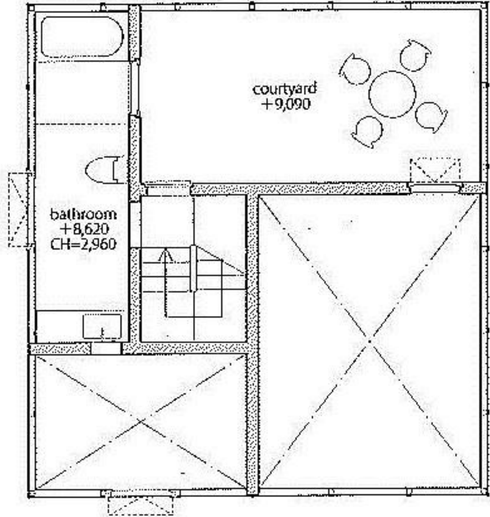
3rd floor plan (upper); scale: 1/150
