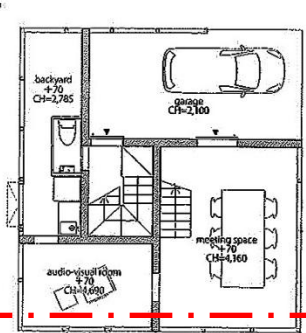
1st floor plan; scale: 1/150
