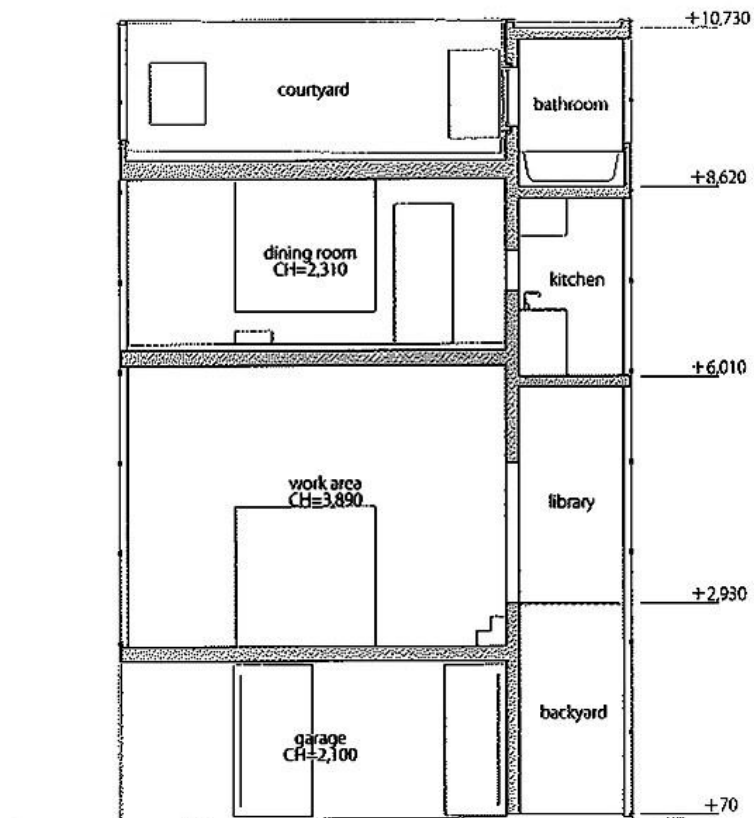
D-D section; scale: 1/150
