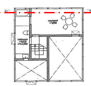
3rd floor plan (upper); scale: 1/150
