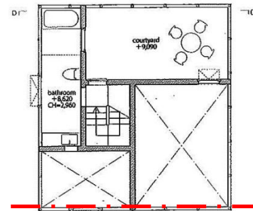
3rd floor plan (upper); scale: 1/150
