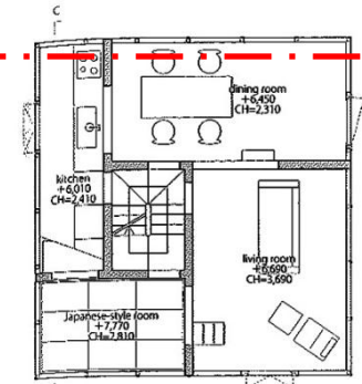
3rd floor plan (lower); scale: 1/150
