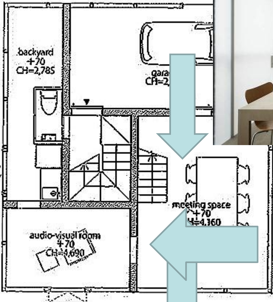
1st floor plan; scale: 1/150
