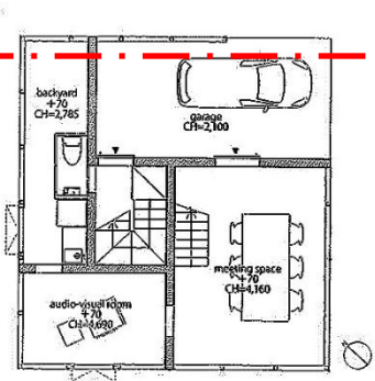
1st floor plan; scale: 1/150
