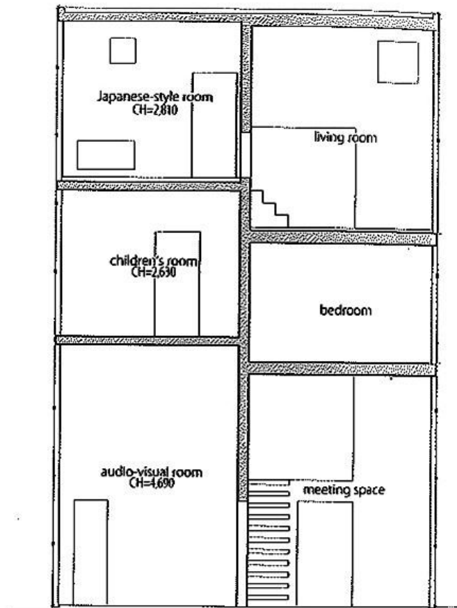
B-B section; scale: 1/150
