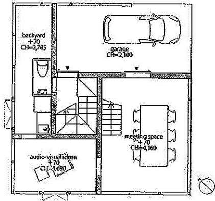
1st floor plan; scale: 1/150
