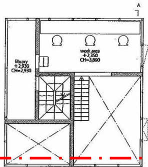
2nd floor plan(lower); scale: 1/150
