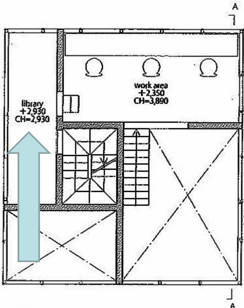
2nd floor plan(lower); scale: 1/150
