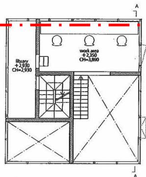
2nd floor plan(lower); scale: 1/150
